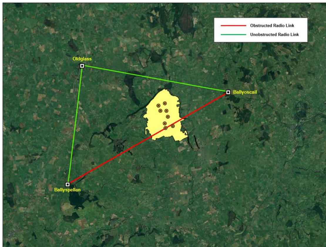
Figure 18. Example of how an existing telecoms mast could be relay the radio link between Ballyspellan and Ballyoscaill.
